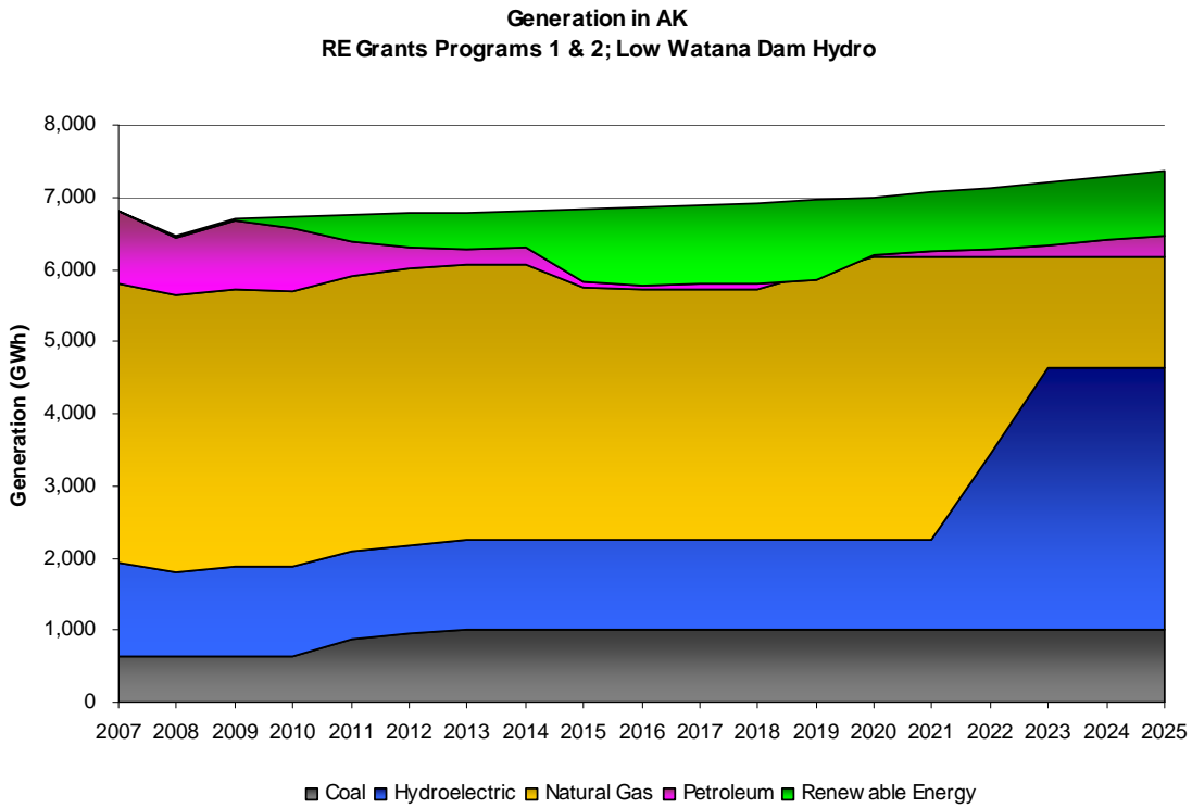
Figure G-6. Fuel mix through 2025 with full implementation of AEA Renewable Energy Grant programs and large hydroelectric project (Low Watana dam equivalent)
