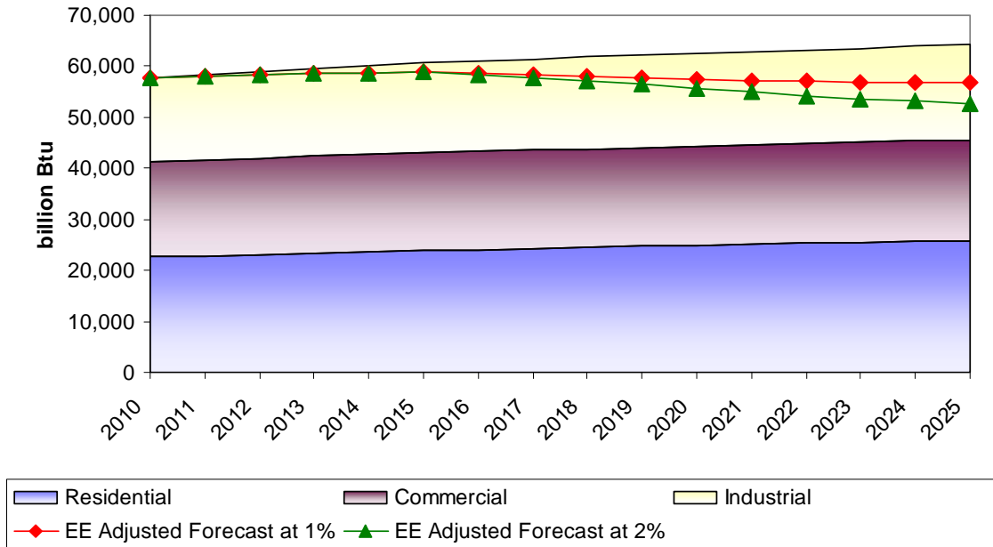
Figure G-2. Natural gas demand forecast with/without energy efficiency scenarios
