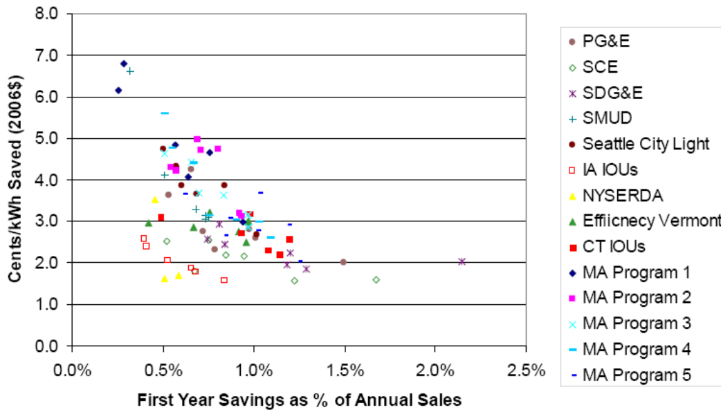
Figure G-4. Utility cost of saved energy for multiple utilities over multiple years 6
